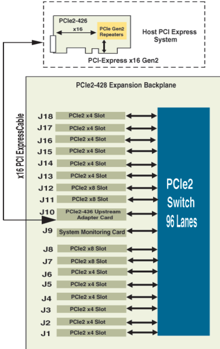
Figure 1-1. PCIe2-2709 Block Diagram
