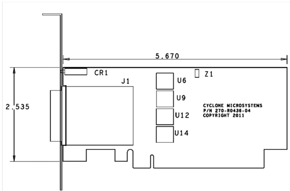
Figure 5-5. PCIe-436 Physical Configuration
