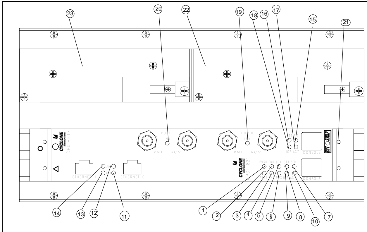
Figure 2-3. 600-2400-30 FEP Front Panel LEDs
