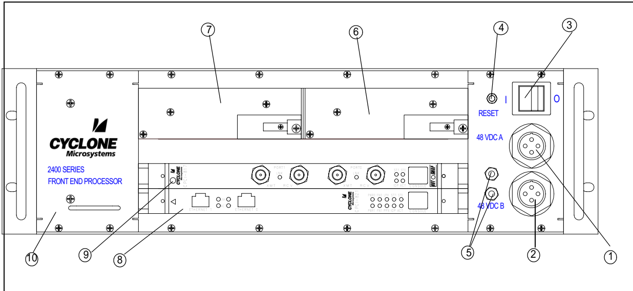
Figure 2-1. 600-2400-30-D0 FEP Front Panel
