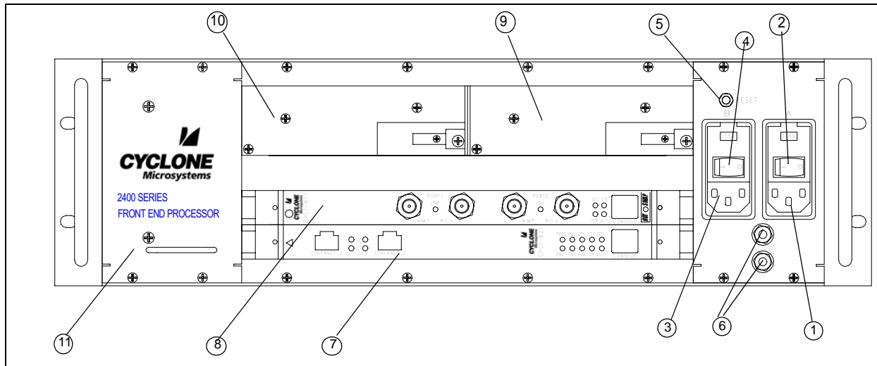
Figure 2-2. 600-2400-30-A0 FEP Front Panel
